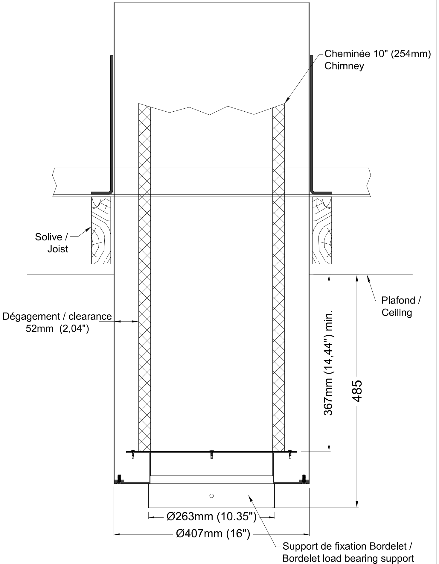
Foyer EVA 992 - Fireplace - Raccord cheminée isolée - 254mm (10") - Connection to insulated chimney
